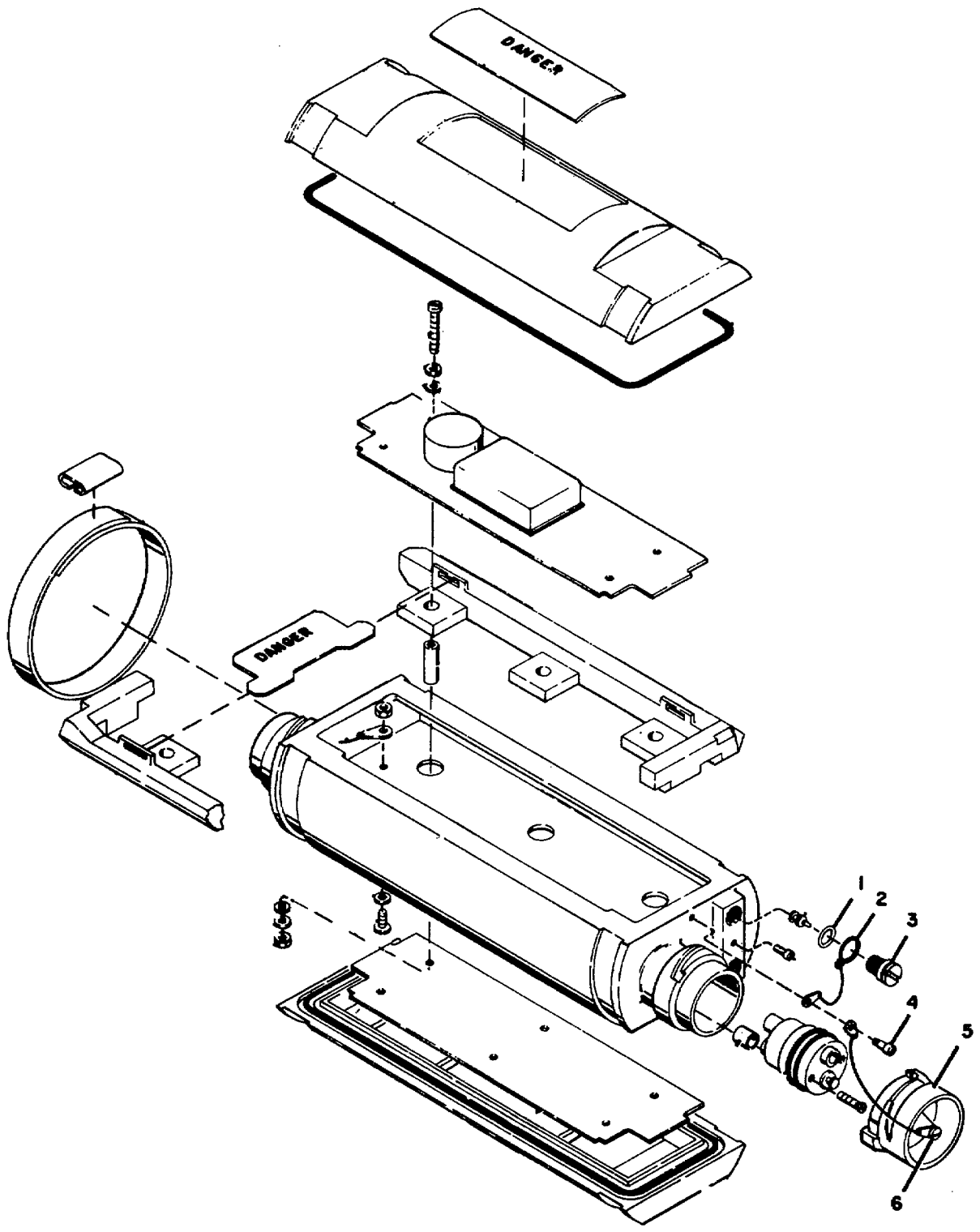
Figure 2. Restorer, Pulse Form TD-206X/G
